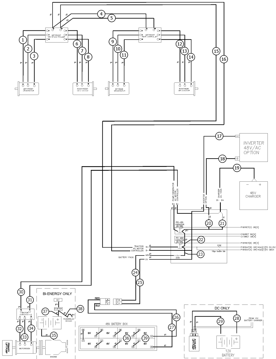
POWER CABLE DIAGRAM S60FE/DC
